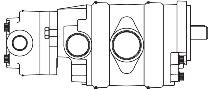
Double Gear Pump with Tandem Backplate
