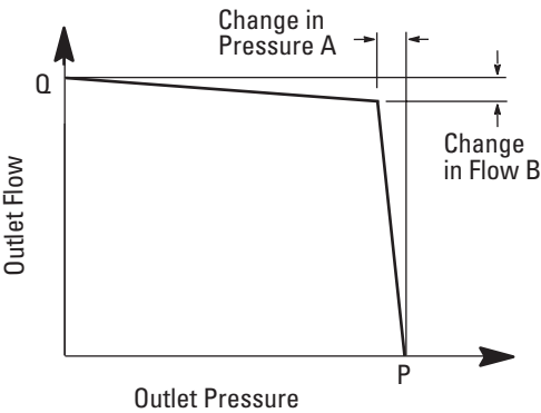
PRESSURE CUT-OFF CHARACTERISTICS OF PRESSURE COMPENSATOR CONTROL @ 49°C (120°F), STATIC CONDITIONS
