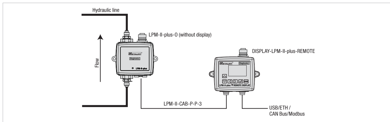
Connection diagram: Remote display
